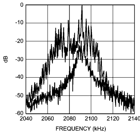
Switching Energy RBW = 300 Hz
